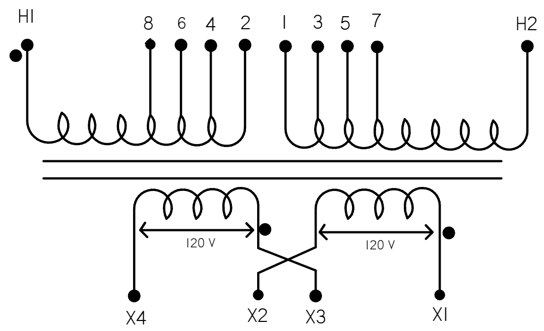
CONNECTION DIAGRAM
