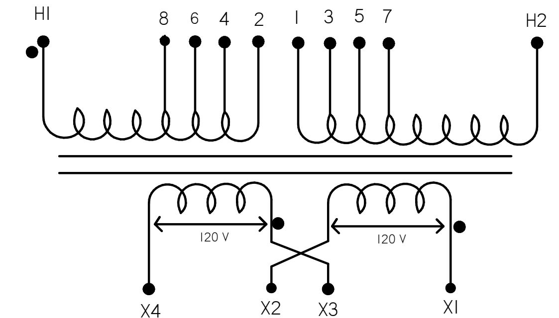
CONNECTION DIAGRAM
