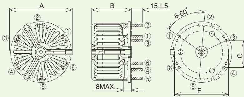
Figure 34. FM□□K□□□MBPF
