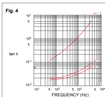
\tan \delta DRIFT VERSUS FREQUENCY LOW VOLTAGE ( \leq 100 V_r d.c.)
