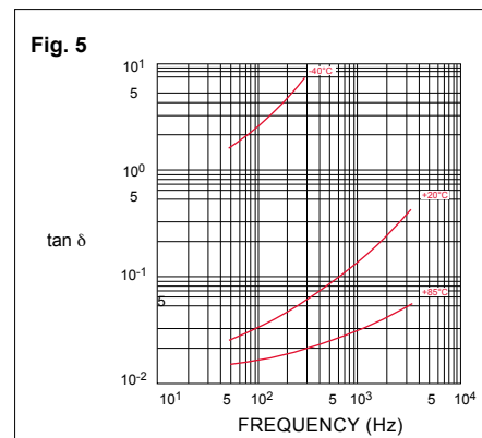
\tan \delta DRIFT VERSUS FREQUENCY HIGH VOLTAGE ( > 100 V_r d.c.)
