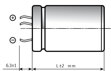
4 PIN CAPACITOR
