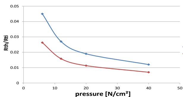
Compression KP 97
