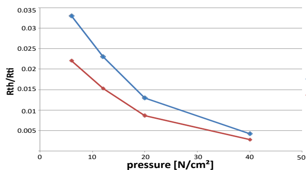
Compression KP 99
