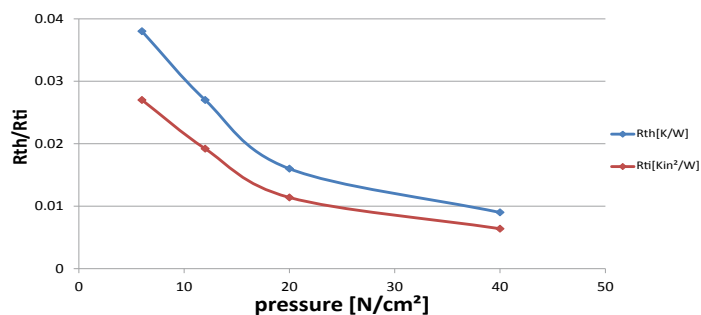
Compression KP 98
