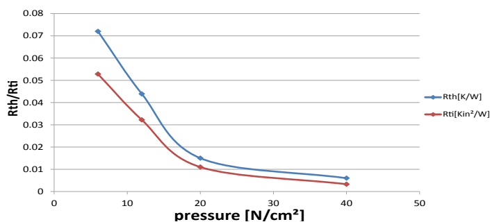
Compression KP 12
